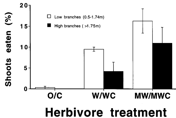
Fig. 1 Rates of shoot herbivory (% shoots eaten) between March and June 1996 across experimental herbivore treatments. Bars are standard errors, based on three blocks. Herbivore treatment classes are based on the large herbivores allowed: O no large mammalian herbivores, C cattle, W native large mammalian herbivores (less megaherbivores), M megaherbivores (giraffes and elephants). Analysis of variance shows significant effects of treatment ( F = 21.7 , P < 0.001 ) and branch height ( F = 4.80 , P < 0.05 ) on browse rates
