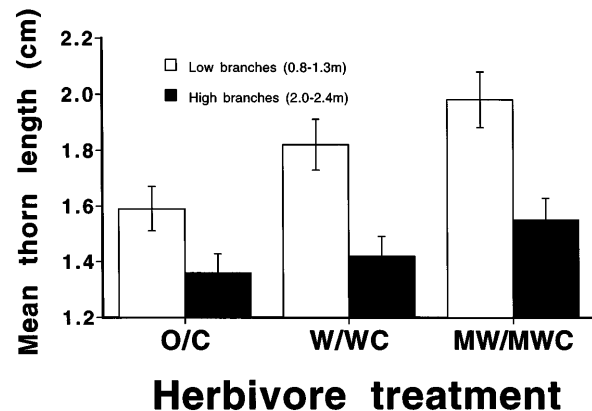
Fig. 2 Mean (untransformed) spine lengths of low (~1.0 m, open bars) and high (~2.2 m, filled bars) branches on Acacia drepanolobium trees accessible to different herbivores. Note scale of vertical axis. Bars are standard errors, based on 120 trees. For statistical analysis, sample size per treatment was 3 (blocks), and the spine lengths were log-transformed. Herbivore treatment classes are based on the large herbivores allowed: O no large mammalian herbivores; C cattle, W native large mammalian herbivores (except megaherbivores), M megaherbivores (giraffes and elephants)
