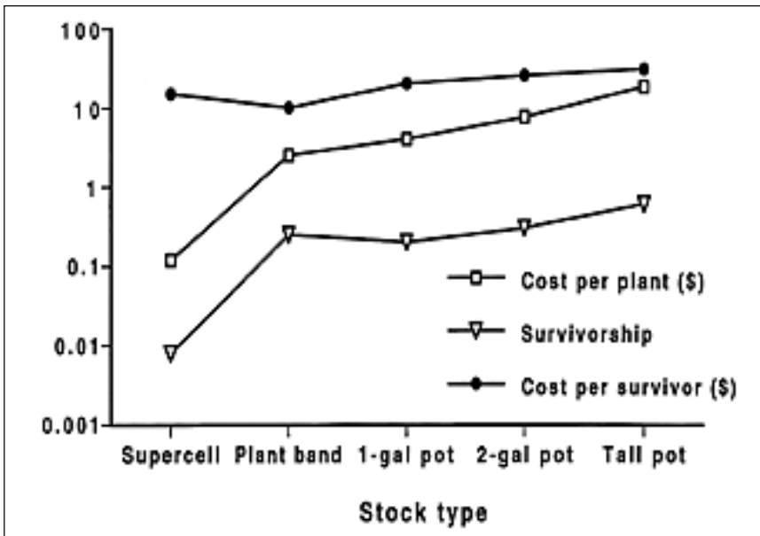
Figure 1. Cost effectiveness of different container stocks in desert restoration sites, estimated across several woody species (adapted from Bainbridge et al., 1995). Although cost per planted seedling varies over more than two orders of magnitude, cost per survivor varies relatively little.
