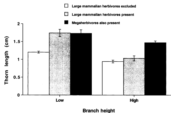
Fig. 1. Mean spine lengths of low (~1 m) and high (~2 m) branches on A. drepanolobium trees accessible to different herbivores. Only trees occupied by the ant C. mimosae were sampled. Bars are standard errors, based on three blocks. For complete sample sizes, see text. Herbivore treatment classes are based on the large herbivores allowed (see Methods).
