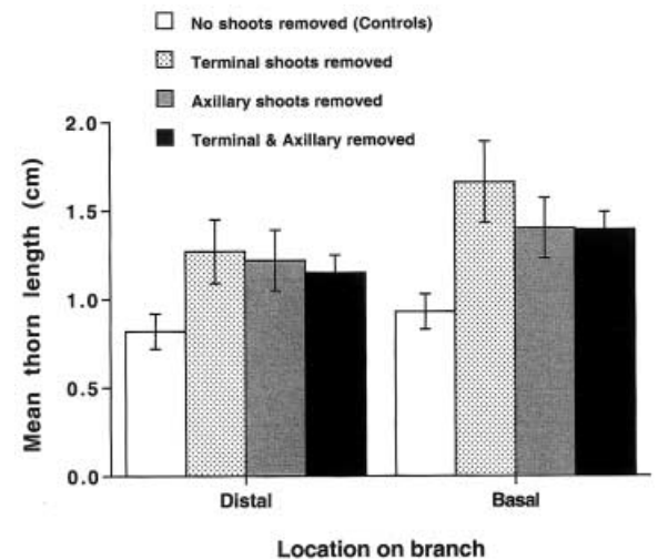
Fig. 4. Mean spine lengths on trees grown in a greenhouse (without either acacia ants or mammalian herbivores) and subjected to different treatments meant to simulate the pruning of axillary and terminal shoots carried out by C. nigriceps . Bars are standard errors.
