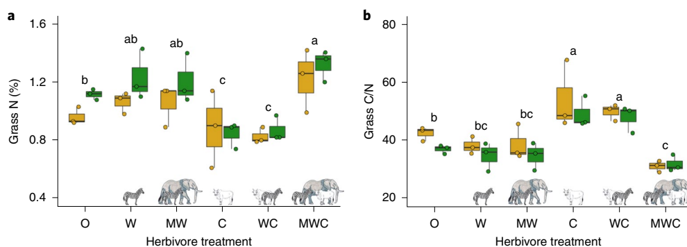
Fig. 3 | Herbivore treatment effects on grass N and C/N ratio. a, b. Impact of herbivore treatments on live grass N concentrations ( a ) and C/N ratio ( b ) outside (golden boxplots and points) and under (green boxplots and points) the canopy of A. drepanolobium trees. Boxplots include the median and their whiskers the minimum and maximum values ( N = 3 ). Herbivore treatments include no large herbivores (O), wild mesoherbivores (W), wild mega- and mesoherbivores (MW), only cattle (C), wild mesoherbivores and cattle (WC) and wild mega- and mesoherbivores and cattle (MWC). Boxplots not sharing the same letter indicate significant differences between herbivore treatments combining sampled locations (outside and under canopy cover), because there was no significant interaction between herbivore treatment and sampled location (results from ANOVA, Table 1).
