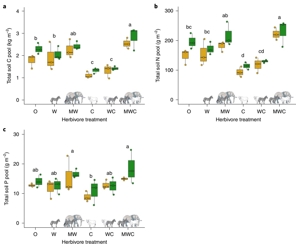
Fig. 2 | Herbivore treatment effects on soil C, N and P pools. a–c , Impact of herbivore treatments on soil C ( a ), N ( b ) and P ( c ) pools outside (golden boxplots and points) and under (green boxplots and points) the canopy of A. drepanolobium trees. Boxplots include the median and their whiskers the minimum and maximum values ( N=3 ). Herbivore treatments include no large herbivores (O), wild mesoherbivores (W), wild mega- and mesoherbivores (MW), only cattle (C), wild mesoherbivores and cattle (WC) and wild mega- and mesoherbivores and cattle (MWC). Boxplots not sharing the same letter indicate significant differences between herbivore treatments combining sampled locations (outside and under the canopy), because there was no significant interaction between herbivore treatment and sampled location (results from analysis of variance (ANOVA), Table 1).
