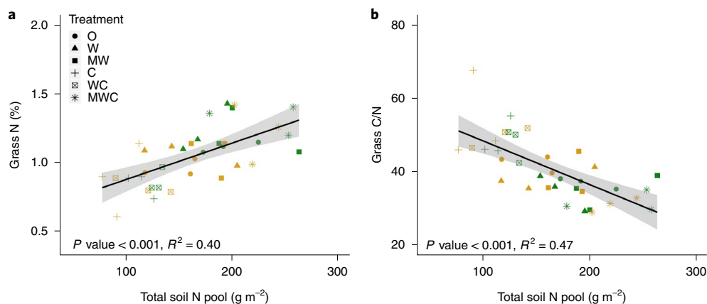
Fig. 4 | Relationship between soil and grass. a,b , Linear regressions showing relationships between total soil N pool and live grass N concentration ( a ) and C/N ratio ( b ). Data were pooled over herbivore treatments and sampled locations. Herbivore treatments include no large herbivores (O), wild mesoherbivores (W), wild mega- and mesoherbivores (MW), only cattle (C), wild mesoherbivores and cattle (WC) and wild mega- and mesoherbivores and cattle (MWC). Sampled locations are outside (golden symbols) and under (green symbols) the canopy of A. drepanolobium trees.
