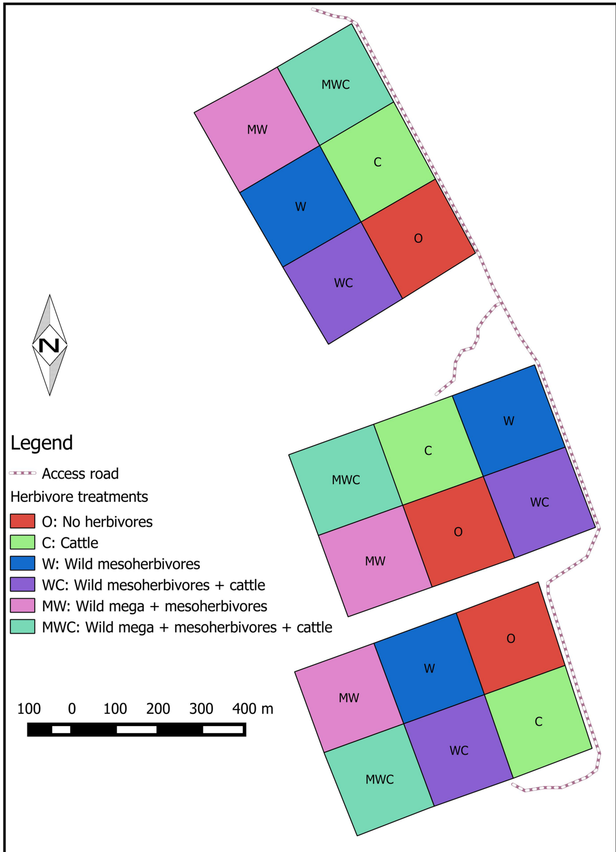
Extended Data Fig. 5 | The Kenya Long-term Exclosure Experiment (KLEE). Schematic of the Kenya Long-term Exclosure Experiment (KLEE) plots. The letters inside each plot indicate the herbivore treatments.
