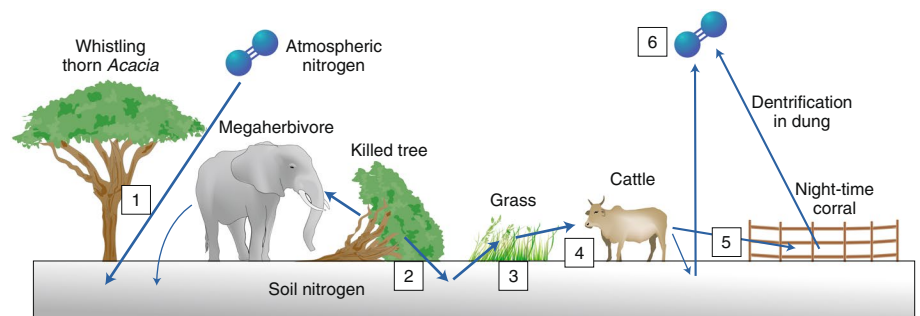
Fig. 1 | Illustration of the savanna nitrogen pump, as implied by the results of Sitters and colleagues. Atmospheric nitrogen ( N_2 ) is fixed by tree symbiotic bacteria (1), cycled into soil N by megaherbivores killing trees (2), taken up by grass (3), eaten by cattle (4) and a portion is removed from the landscape to night-time corrals (5). Organic forms of N in dung and soil are converted to N_2 (6) by microbes, in a process called denitrification, to complete the cycle. Without megaherbivores, the cycle is interrupted and soil N and C outside corrals are depleted.
