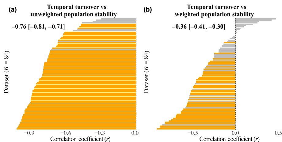
Fig. 4 Histograms of the correlation coefficients ( r ) for each dataset between temporal turnover and unweighted population stability (a), and weighted population stability (b). All the variables were ln-transformed. Significant positive, significant negative, and nonsignificant correlations are represented by blue, orange, and gray colors, respectively. Mean correlation coefficients ( \bar{r} ) and 95% confidence intervals from linear mixed-effects models are also shown within each panel.
